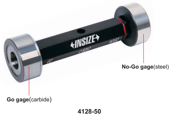
Size tolerance of H7 (mm)
